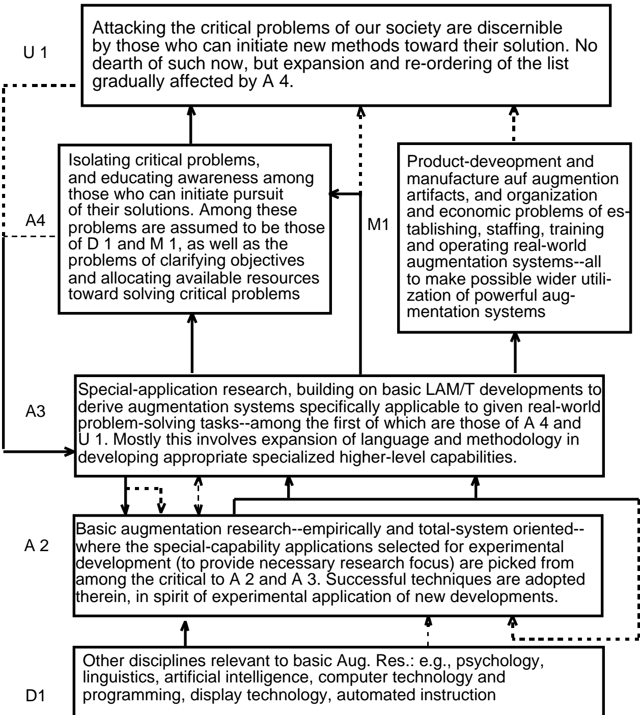
Fig. 5: A Total Program
